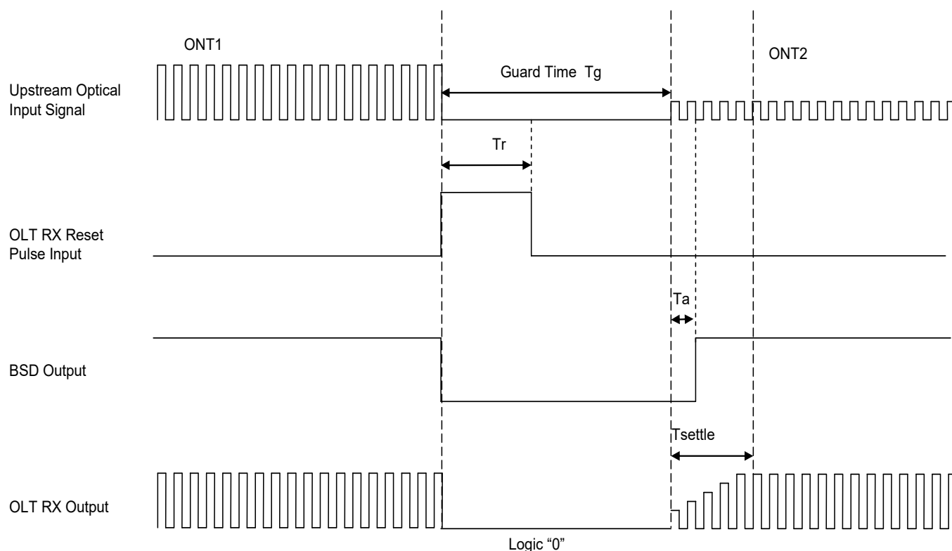
LTE3680P Timing Diagram
